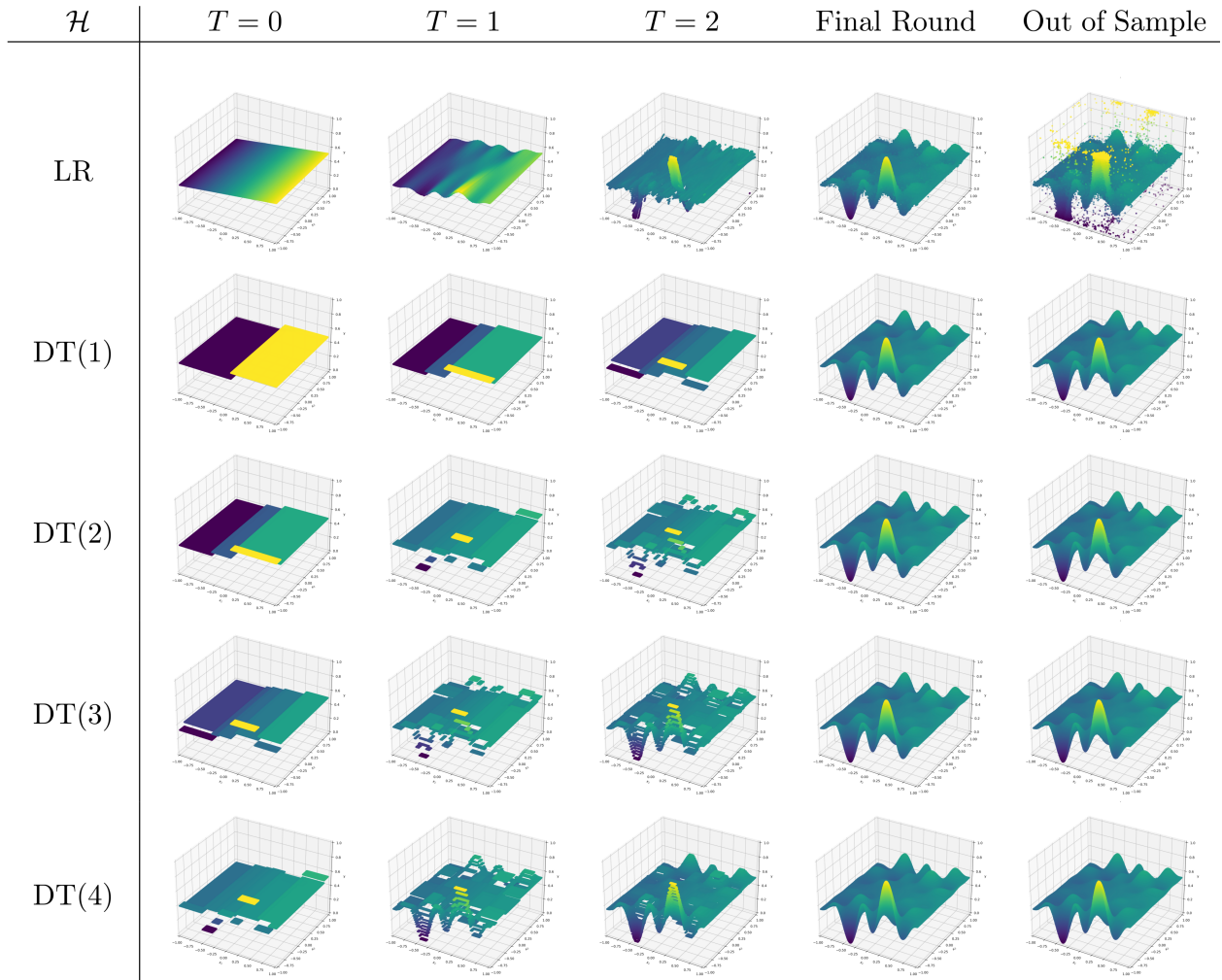
Figure 4: Stages of Algorithm 1 learning C_1 with linear regression (LR) and varying depth d decision trees (DT( d )). In the out of sample plot for linear regression, points are not mapped to their proper position, implying C_1 cannot be learned by boosting linear functions. All other hypothesis classes eventually converge to C_1 .
